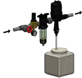
inline installation
